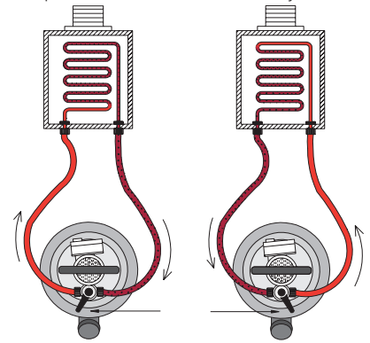
fig. 1 - Clockwise circulation
